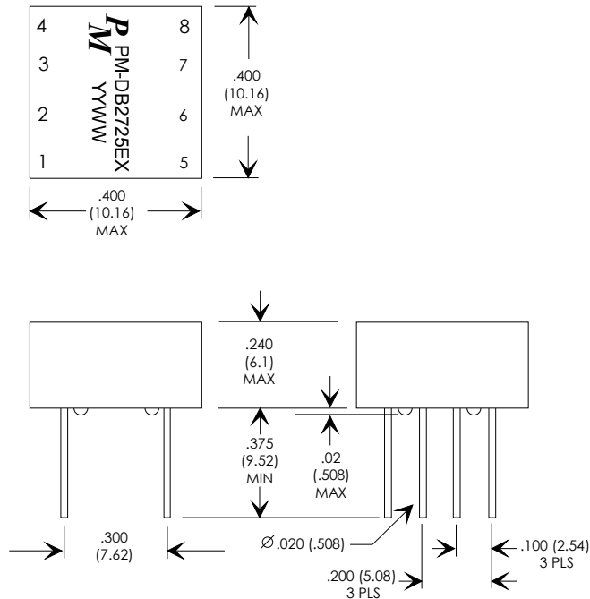
FIGURE 2: PHYSICAL DIMENSIONS IN INCHES (mm)
